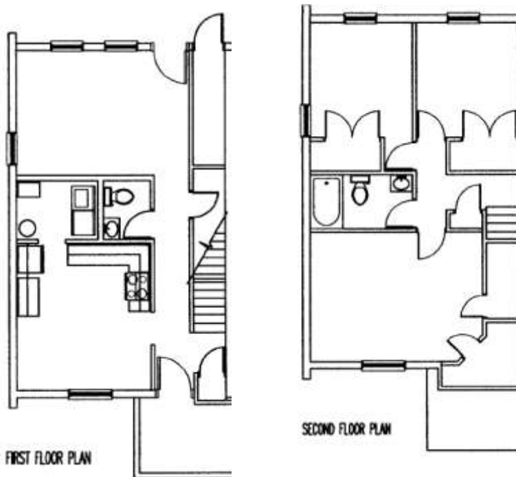
Three-Bedroom Floor Plan
