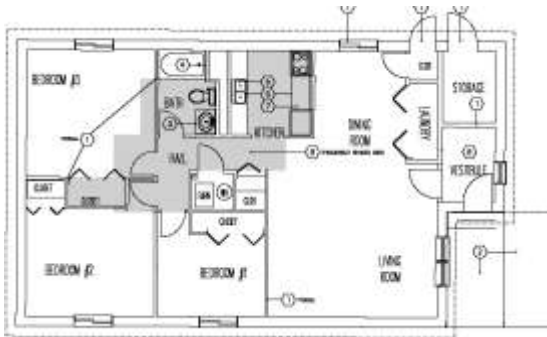
Three-Bedroom Ranch Floor Plan
