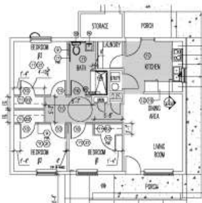
Three-Bedroom Ranch Physically Accessible Floor
